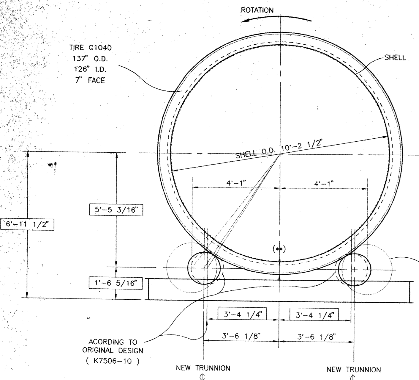
FEED AND DISCHARGE END TRUNNION ROLL DETAILS ( SECTIONS A-A & B-B )
