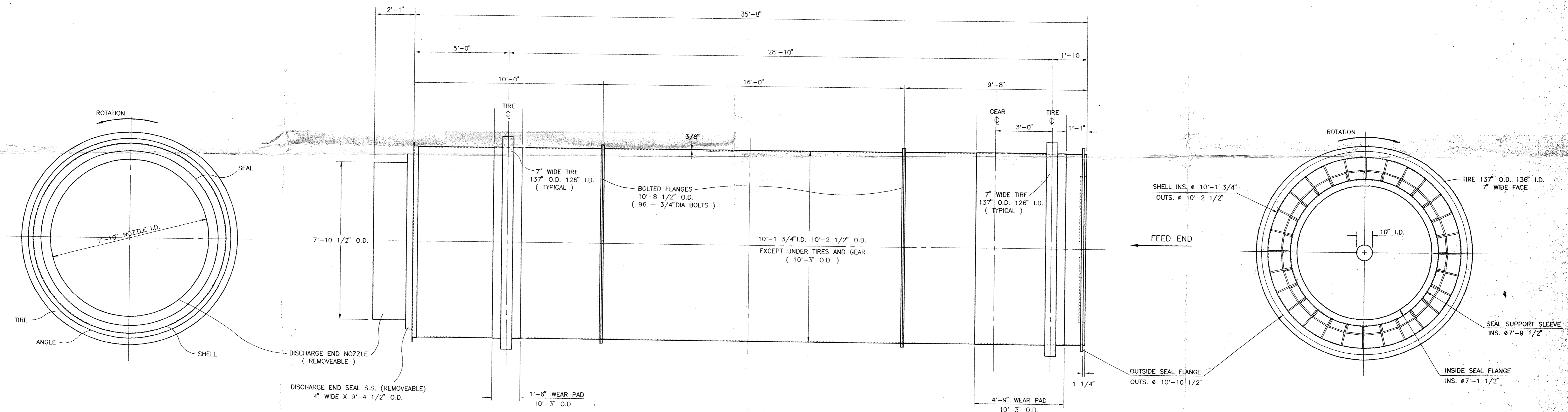
LEFT END VIEW ( DISCHARGE END )
